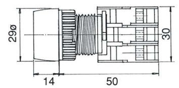
GEPFL22-10/C Push ON-Push OFF
