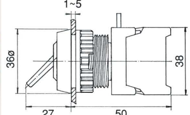
LS30-1/O , 0-1 , LS30-1O/C , 1-2 LS30-2/O , 0-1
