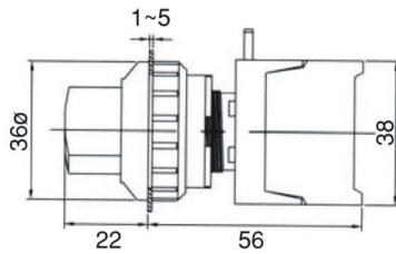
SRL30-1/O , 0←1 , Spring return SRL30-1/C , 1←0 , Spring return
