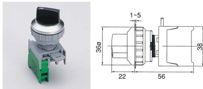
SS30-1O/C 1-2
