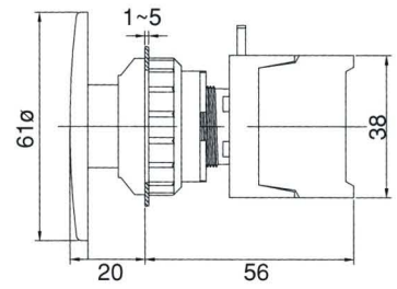
XLEB30-1/C Latching STOP
