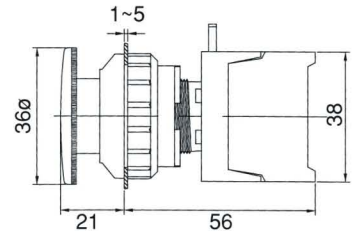
XLEB30-1O/C Latching STOP
