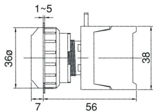
EPFL30-1O/C Push ON-Push OFF
