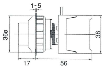
PFL30-1O/C Push ON-Push OFF
