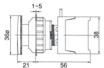
XLEB30-1O/C Latching STOP
