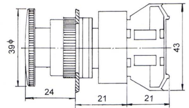
ILLUMINATED PUSH BUTTON NLPB 25-1O/C
