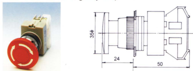
ALEPB 22-1/C Emergency stop
