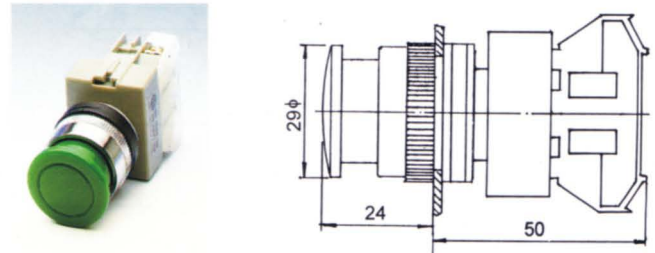
AEPBS 22-1/O, AEPBS22-1/C
