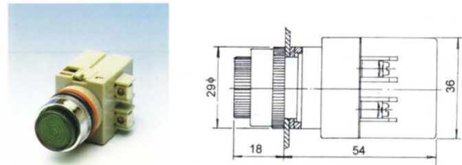
TPL-22 TRANSFORMER PILOT LIGHT TPL-25
